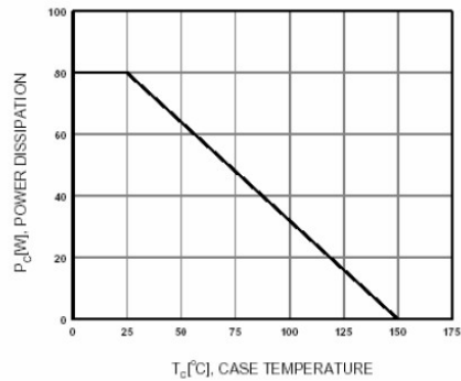
Figure 6. Power Derating
