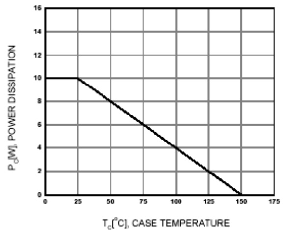
Figure 8. Power Derating
