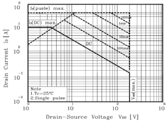
Figure 9-2. Maximum Safe Operating Area for TO-220F
