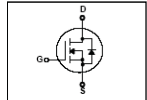
HFD5N65U
